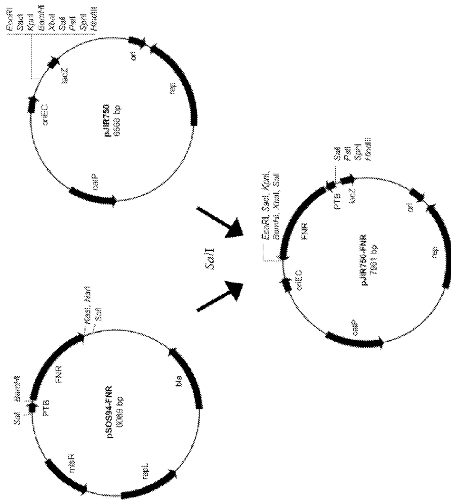
FIGURE 4: PLASMID MAPS
