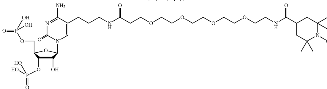
TEMPO-PEG 4 -Alkane-3',5'-Bisphosphate-Cytidine (TP 4 A-3',5'-pCp)
