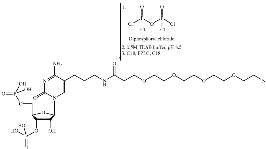
10 MW = 733.55 Azido-PEG 4 -Alkane-3',5'-Bisphosphate-Cytidine (AzP 4 A-3',5'-pCp)
