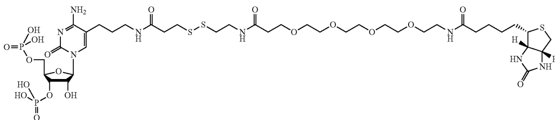
12 MW = 1097.12 Biotin-PEG 4 -SS-Alkane-3',5'-Bisphosphate-Cytidine (BP 4 SSA-3',5'-pCp)
