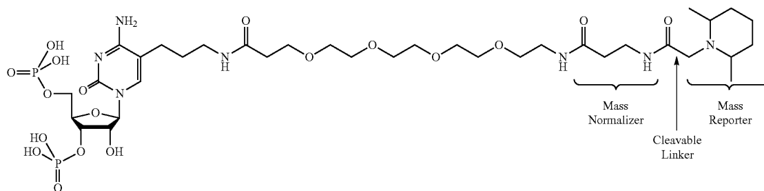
TMT-PEG 4 -Alkane-3',5'-Bisphosphate-Cytidine (TMTp 4 A-3',5'-pCp)
