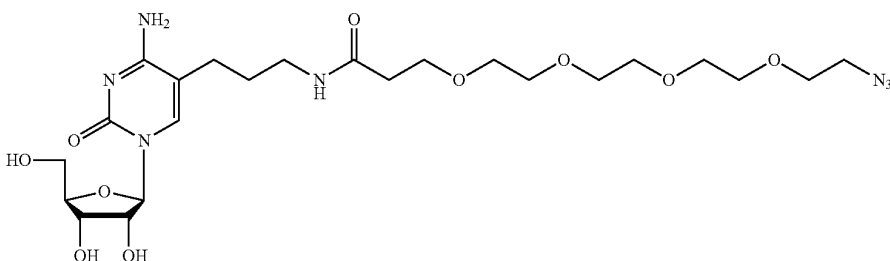
9 MW = 573.59 Azido-PEG 4 -Alkane-Cytidine (AzP 4 AC)
