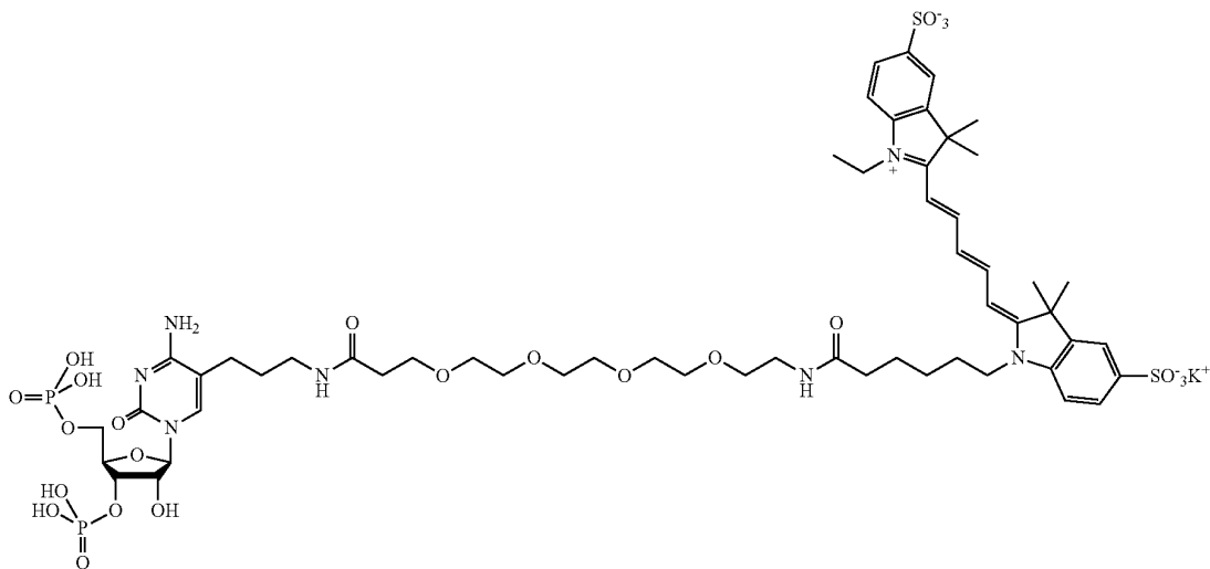
Cy5-PEG 4 -Alkane-3',5'-Bisphosphate-Cytidine (Cy5P 4 A-3',5'-pCp)
