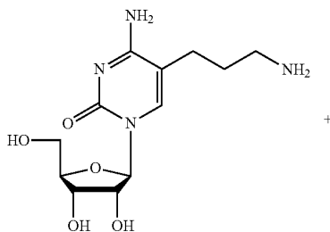
4 MW = 300.31 5-(3-aminopropyl)cytidine
