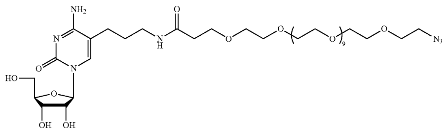
18 MW = 926.02 Azido-PEG 12 -Alkane-Cytidine (AzP 12 AC)
