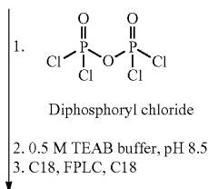
11 MW = 937.16 Biotin-PEG 4 -SS-Alkane-Cytidine (BP 4 SSAC)
