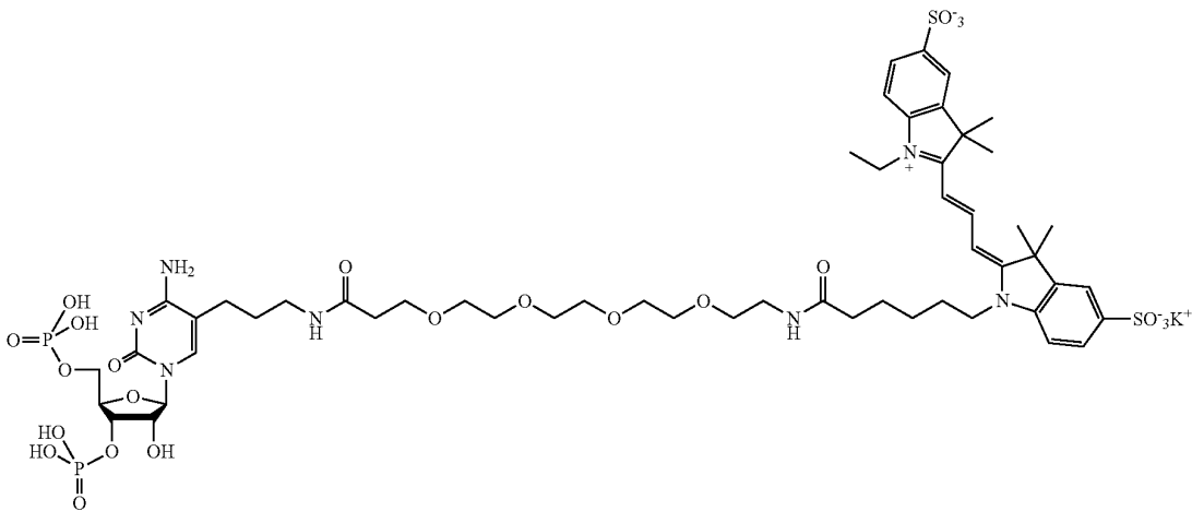
Cy3-PEG 4 -Alkane-3',5'-Bisphosphate-Cytidine (Cy3P 4 A-3',5'-pCp)
