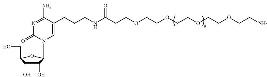
19 MW = 900.02 Amino-PEG 12 -Alkane-Cytidine (AmP 12 AC)
