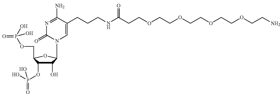
13 MW = 707.56 Amino-PEG 4 -Alkane-3',5'-Bisphosphate-Cytidine (AmP 4 A-3',5'-pCp)
