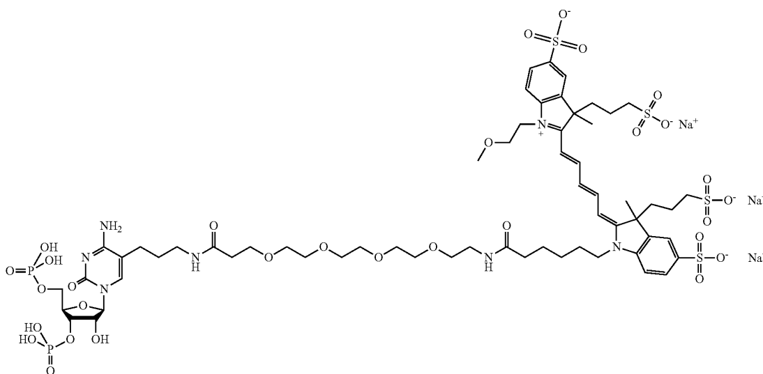
DyLight650-PEG 4 -Alkane-3',5'-Bisphosphate-Cytidine (Dy650P 4 A-3',5'-pCp)
