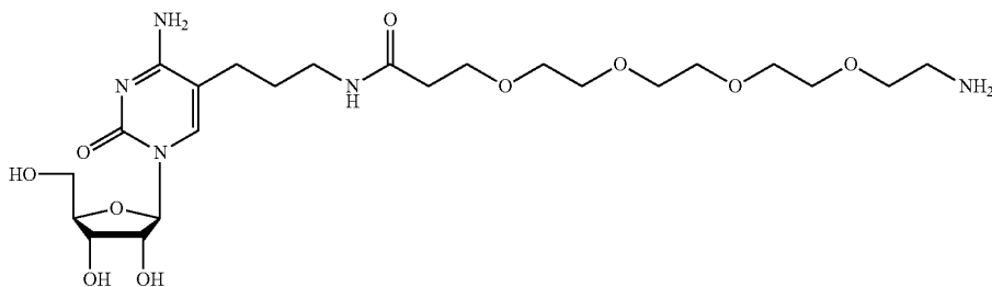
15 MW = 547.60 Amino-PEG 4 -Alkane-Cytidine (AmP 4 AC)
