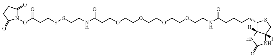
MW = 751.93 NHS-SS-PEG 4 -Biotin
