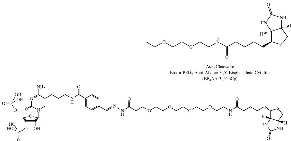
Hydrazone Exchange Cleavable Biotin-PEG 4 -Hydrazone-Alkane-3',5'-Bisphosphate-Cytidine (BP 4 HA-3',5'-pCp)
