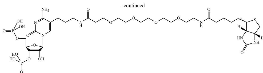
6 MW = 933.85 BPA-3',5'-pCp
