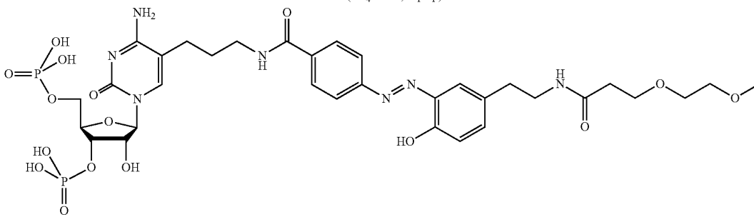
Photo-cleavable Biotin-PEG 4 -Photo-Alkane-3',5'-Bisphosphate-Cytidine (BP 4 PA-3',5'-pCp)
