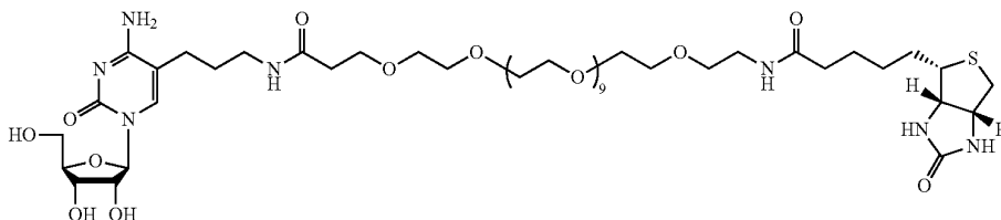
7 MW = 1126.31 Biotin-PEG 12 -Alkane-Cytidine (BP 12 AC)
