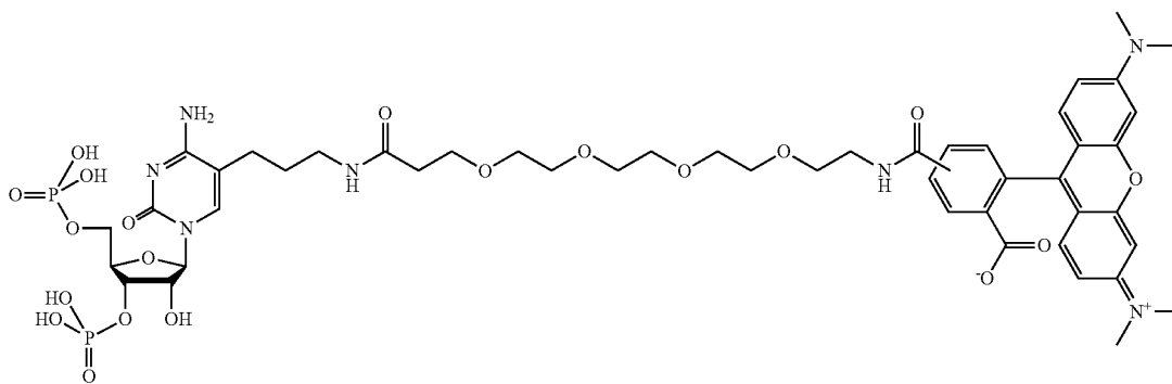
5/6-Carboxytetramethylrhodamine-PEG 4 -Alkane-3',5'-Bisphosphate-Cytidine (5/6-RP 4 A-3',5'-pCp)
