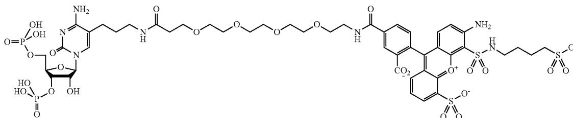
DyLight488-PEG 4 -Alkane-3',5'-Bisphosphate-Cytidine (Dy488P 4 A-3',5'-pCp)
