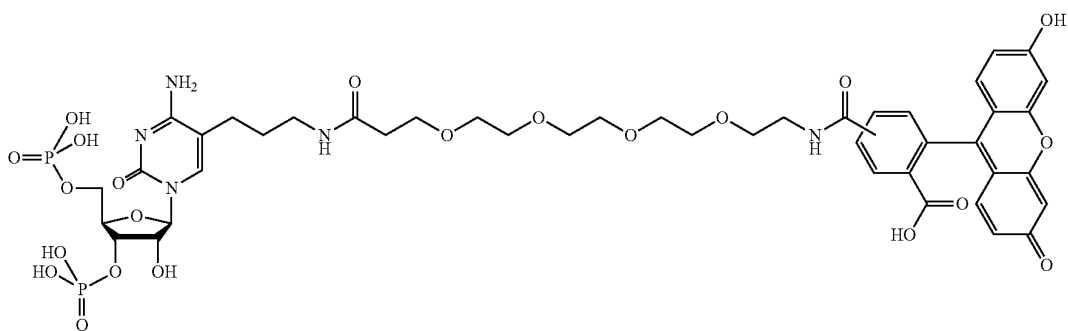
5/6-Carboxyfluorescein-PEG 4 -Alkane-3',5'-Bisphosphate-Cytidine (5/6-FP 4 A-3',5'-pCp)
