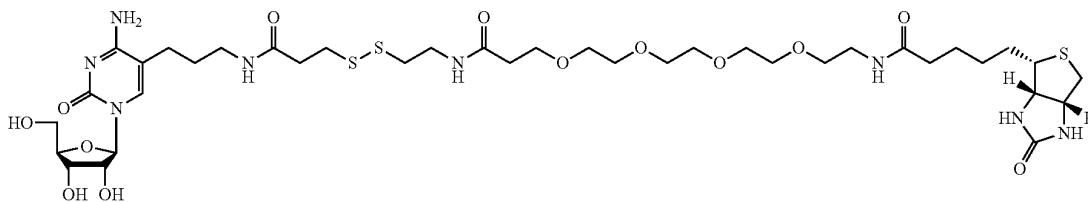
11 MW = 937.16 Biotin-PEG 4 -SS-Alkane-Cytidine (BP 4 SSAC)
