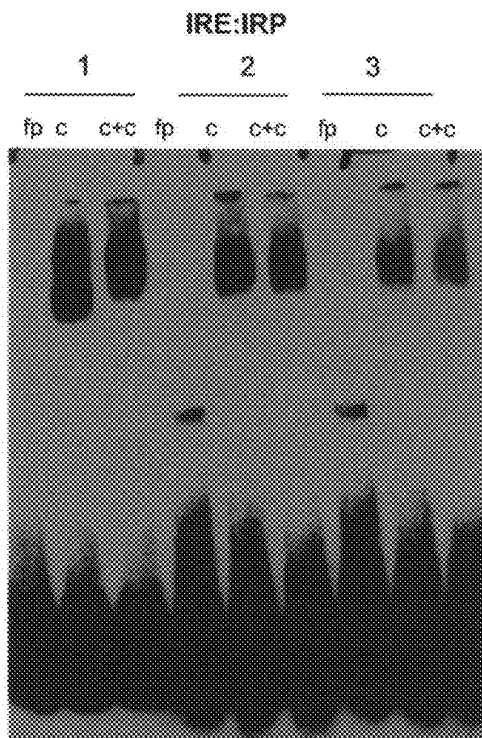
3',5'-Bisphosphorylated Cytidine-Alkene-LC-Biotin
