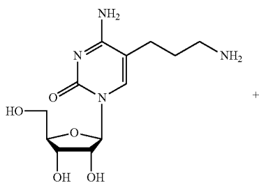
4 MW = 300.31 5-(3-aminopropyl)cytidine
