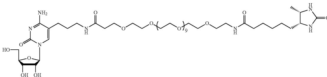
20 MW = 1096.27 Desthiobiotin-PEG 12 -Alkane-Cytidine (DP 12 AC)
