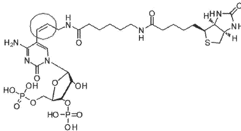
3',5'-Bisphosphorylated Cytidine-Alkene-LC-Biotin
