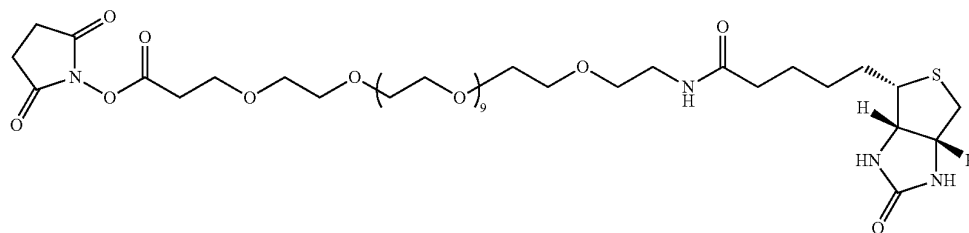
MW = 941.09 NHS-PEG 12 -Biotin
