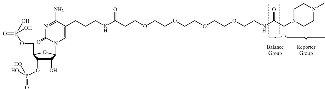
iTRAQ-PEG 4 -Alkane-3',5'-Bisphosphate-Cytidine (iTRAQp 4 A-3',5'-pCp)
