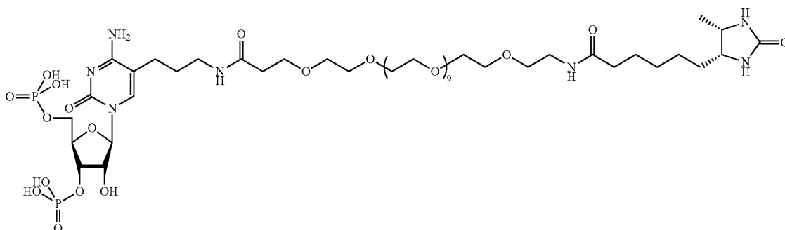
Desthiobiotin-PEG 12 -Alkane-3',5'-Bisphosphate-Cytidine (DP 12 A-3',5'-pCp)
