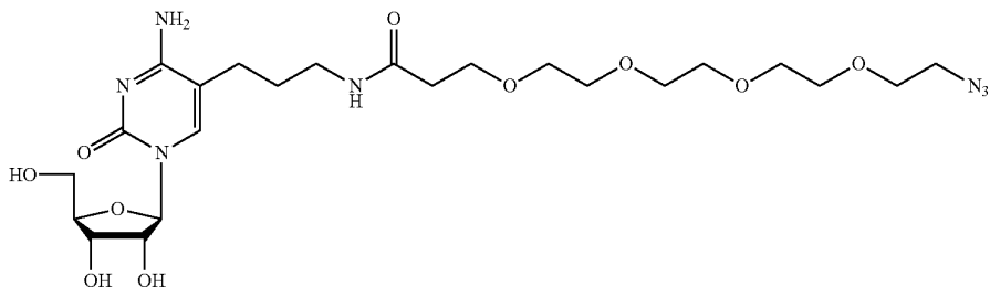
9 MW = 573.60 Azido-PEG 4 -Alkane-Cytidine (AzP 4 AC)
