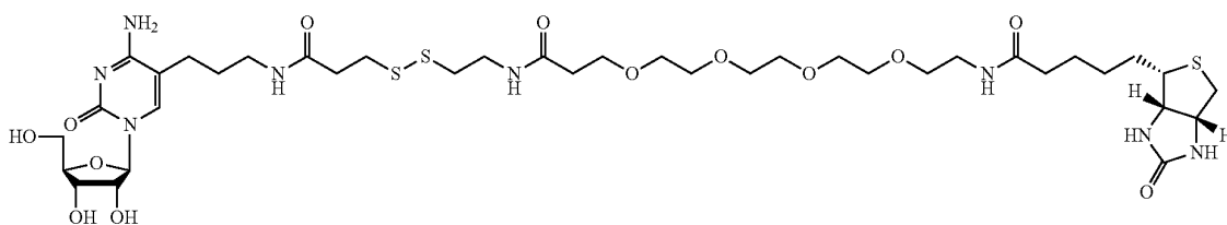
11 MW = 937.16 Biotin-PEG 4 -SS-Alkane-Cytidine (BP 4 SSAC)
